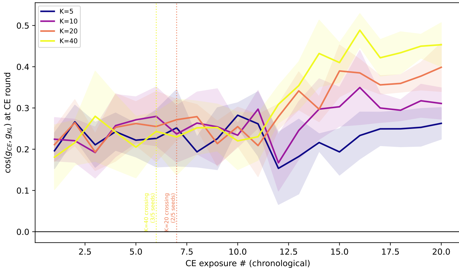
Repeated short-cycle: full cosine trajectory across CE exposures
